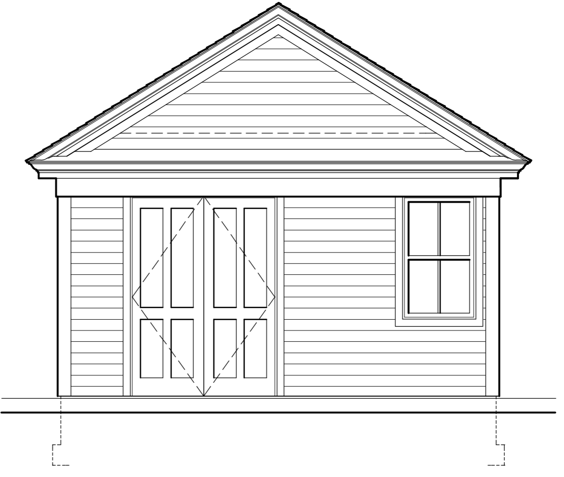
3 POOL HOUSE RIGHT SIDE ELEVATION SK-2 SCALE: 1/4" = 1'-0"
